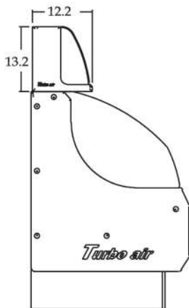
TOM-L COMBINATION WITH TOMD-L SIDE VIEW
