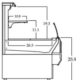
TOM-L SIDE VIEW
