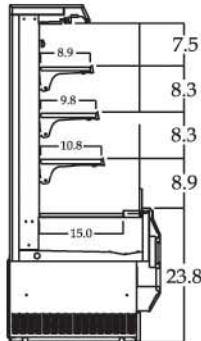
TOM-40M/50M SIDE VIEW
