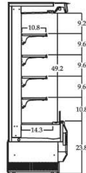
TOM-40/50 SIDE VIEW
