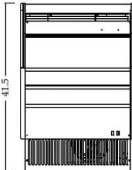
TOM-30S FRONT VIEW
