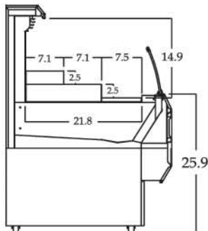
TOM-S SIDE VIEW
