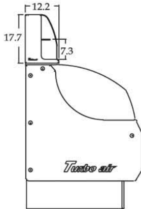
TOM-S COMBINATION WITH TOMD-H SIDE VIEW
