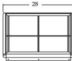
TOMD-30-H PLAN VIEW
