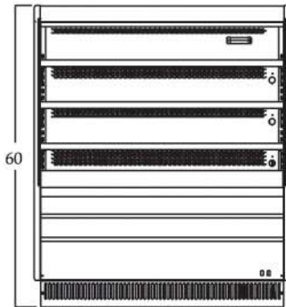
TOM-50M FRONT VIEW
